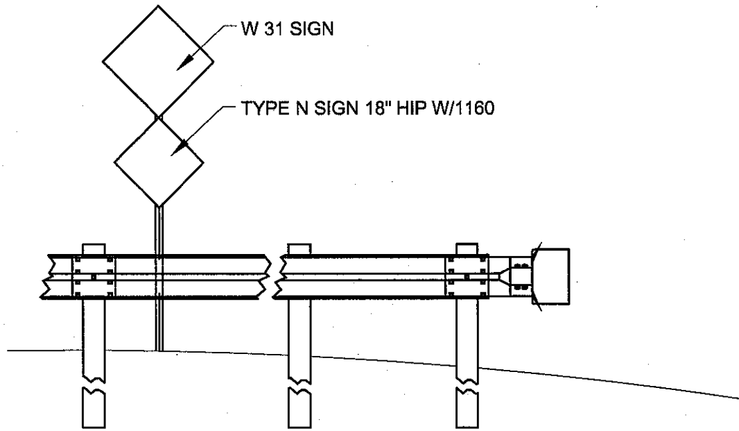
ELEVATION OF BARRICADE
