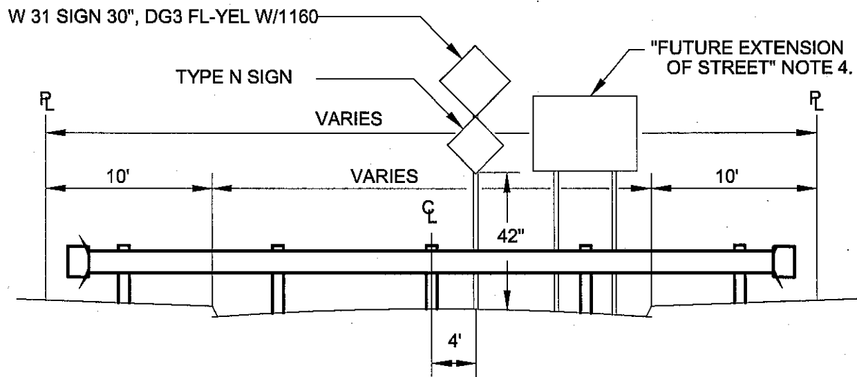
TYPICAL INSTALLATION
